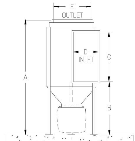
DLF-508 Stainless Steel Left Hand Inlet
